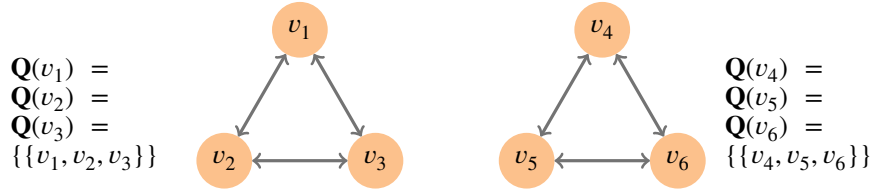
Fig. 6. FBAS lacking quorum intersection
